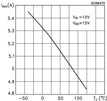
Figure 28. Normalized current limit vs. junction temperature
