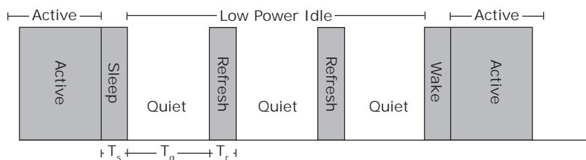
Figure 18 • Low Power Idle Operation
