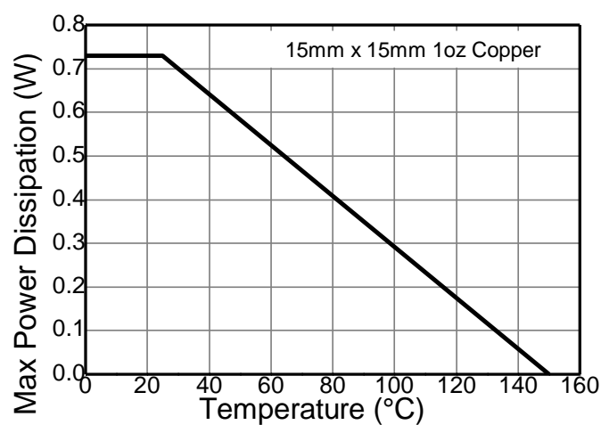
Derating Curve
