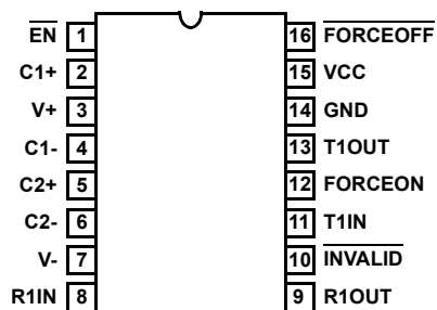
ICL3221E (16 LD SSOP, TSSOP) Top View
