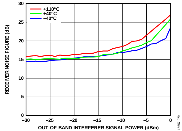
Figure 138. Receiver Noise Figure vs. Out of Band Interferer Signal Power, 3614 MHz LO, 3665 MHz CW Interferer, Noise Figure Integrated over 7 MHz to 10 MHz
