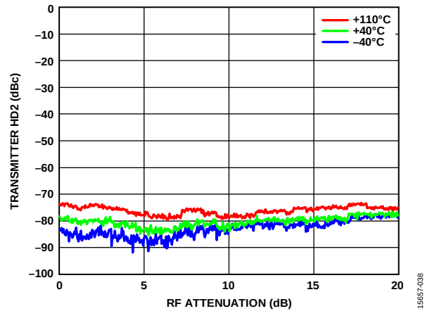
Figure 97. Transmitter HD2 vs. RF Attenuation, 2600 MHz LO, 2605 MHz CW Desired Signal, 40 MHz RF Bandwidth, 245.76 MSPS Sample Rate
