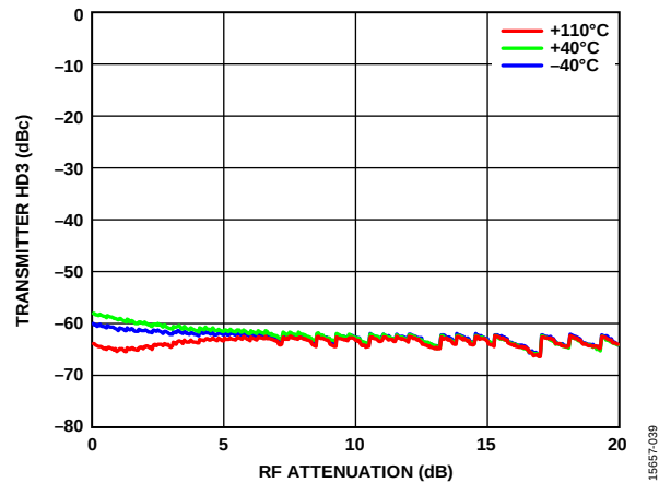
Figure 98. Transmitter HD3 vs. RF Attenuation, 2600 MHz LO, 2605 MHz CW Desired Signal, 40 MHz RF Bandwidth, 245.76 MSPS Sample Rate
