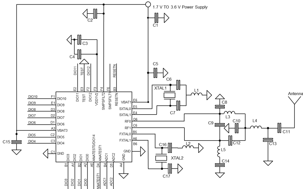
Figure 28. Application circuit: non active DC-DC converter WSP34 package
