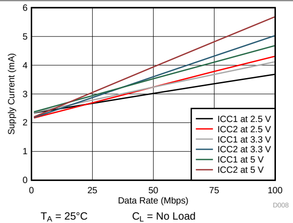
Figure 8. ISO7731-Q1 Supply Current vs Data Rate (With No Load)
