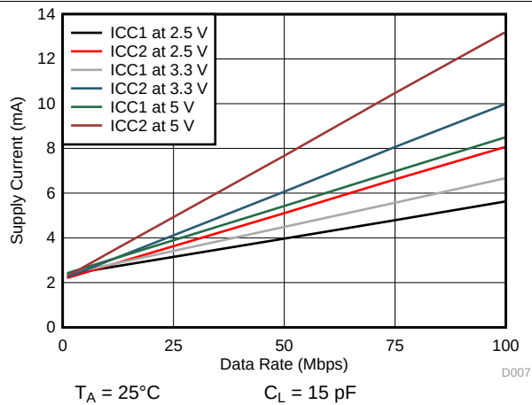
Figure 7. ISO7731-Q1 Supply Current vs Data Rate (With 15-pF Load)
