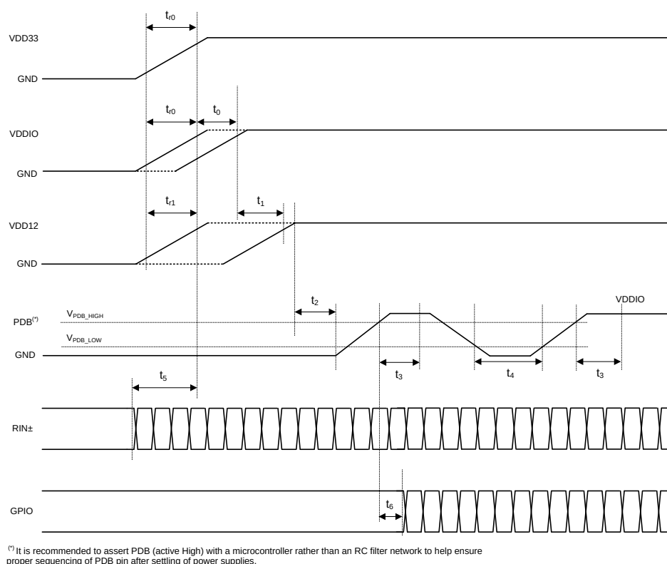
Figure 45. Power-Up Sequencing
