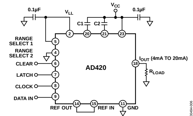
Figure 6. Standard Configuration
