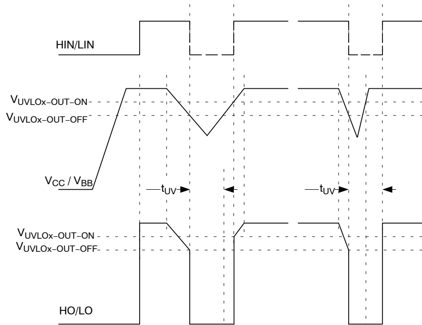
Figure 5. UVLO
