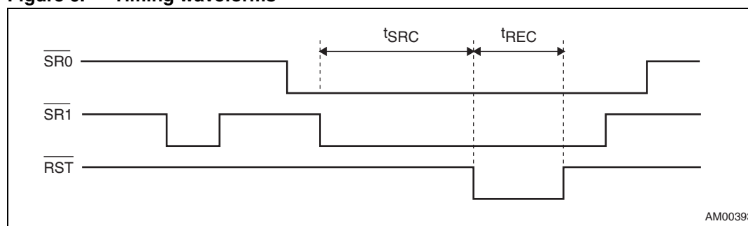
Figure 6. Timing waveforms
