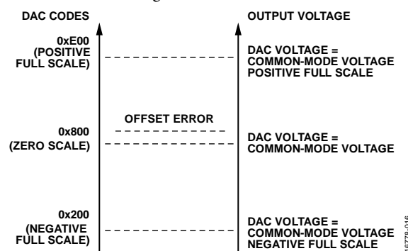
Figure 28. High Speed DAC Transfer Function
