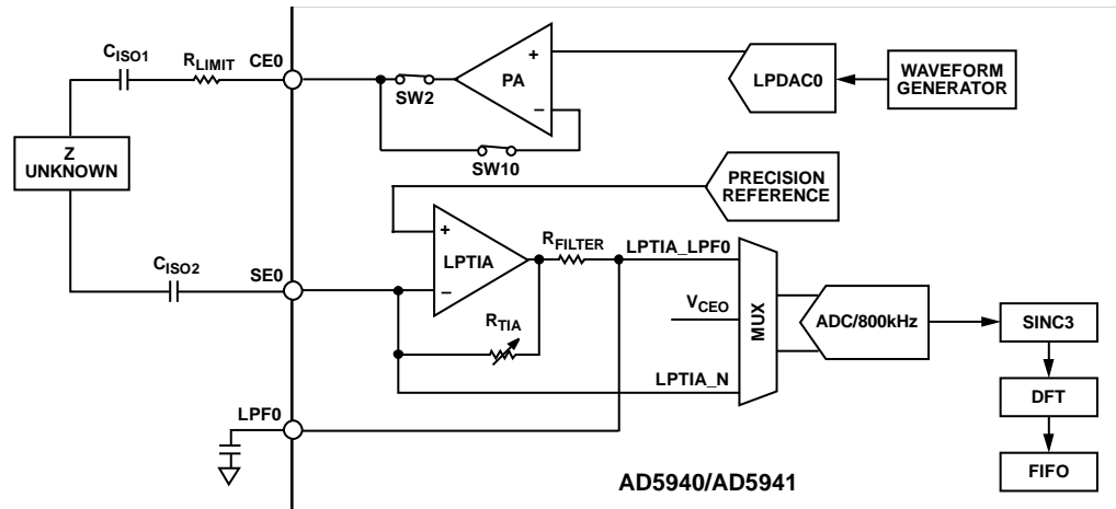
Figure 55. Low Frequency, 2-Wire, Bioimpedance Loop (Maximum Bandwidth = 300 Hz)
