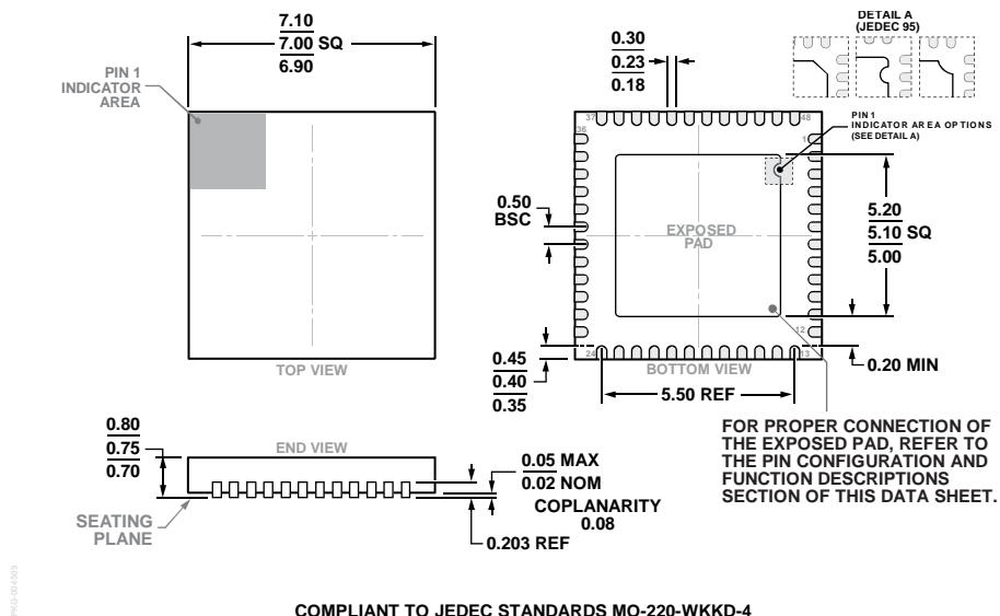
Figure 61. 48-Lead Lead Frame Chip Scale Package [LFCSP] 7 mm × 7 mm Body and 0.75 mm Package Height (CP-48-4)
