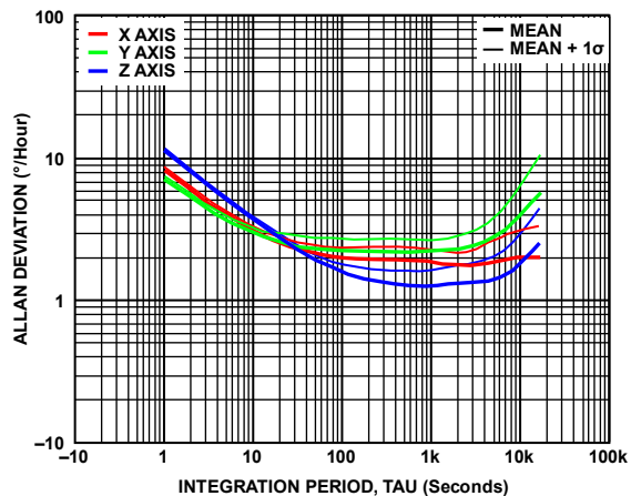
Figure 8. Gyroscopic Allan Deviation, T_C = 25^\circ\text{C} , ADIS16505-2, Plot Taken After 10 Hours of Settling Time
