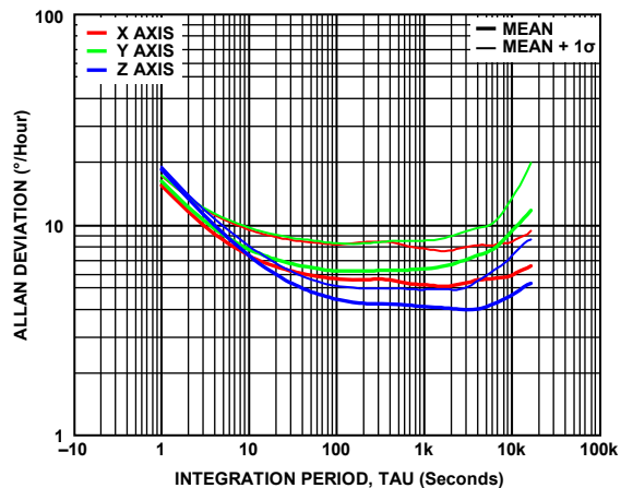
Figure 9. Gyroscopic Allan Deviation, T_C = 25^\circ\text{C} , ADIS16505-3, Plot Taken After 10 Hours of Settling Time
