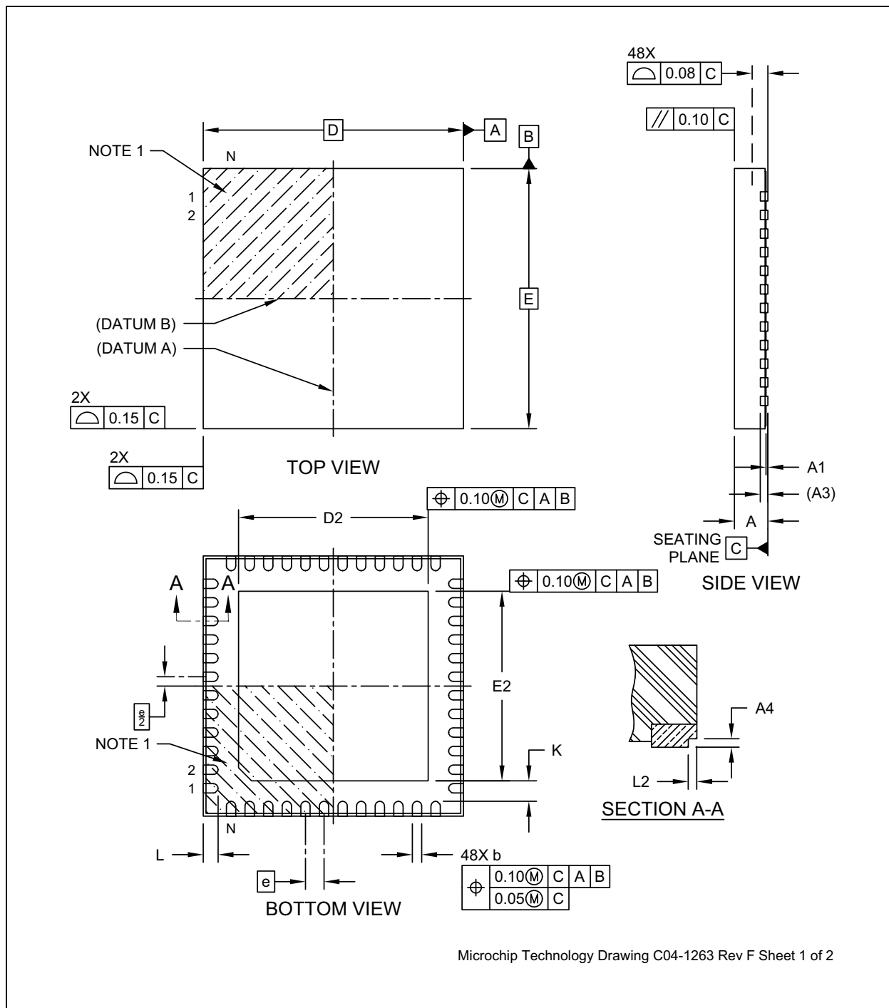
FIGURE 7-4: 48-LEAD VERY THIN PLASTIC QUAD FLAT NO LEAD PACKAGE (PUA) - 7X7 MM BODY (VQFN) WITH 5.05X5.05 MM EXPOSED PAD AND STEPPED WETTABLE FLANKS SHEET 1
