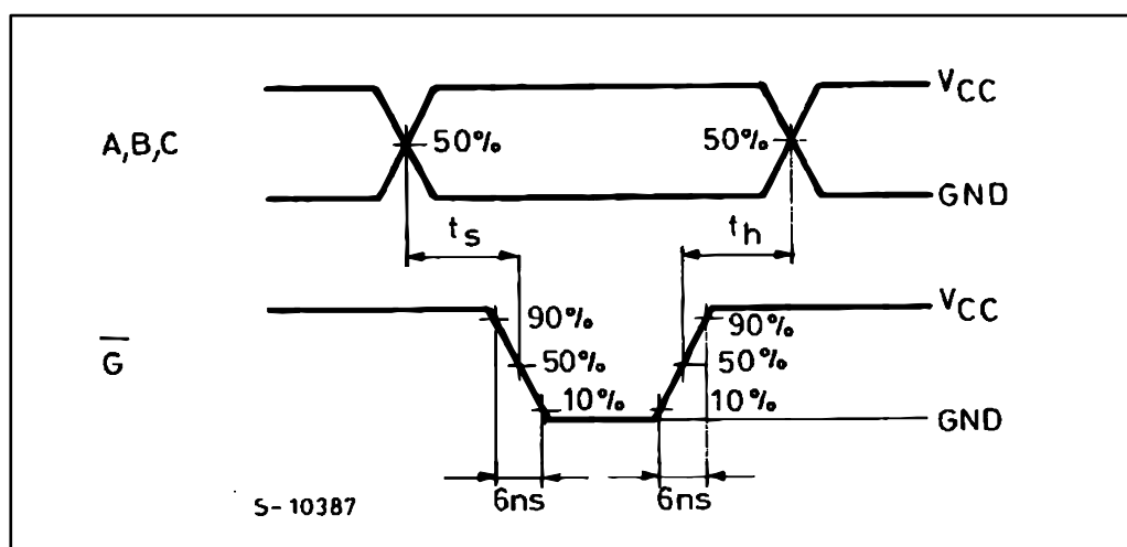
Figure 9: Waveform 5: setup and hold time ( f = 1\text{ MHz} ; 50% duty cycle)
