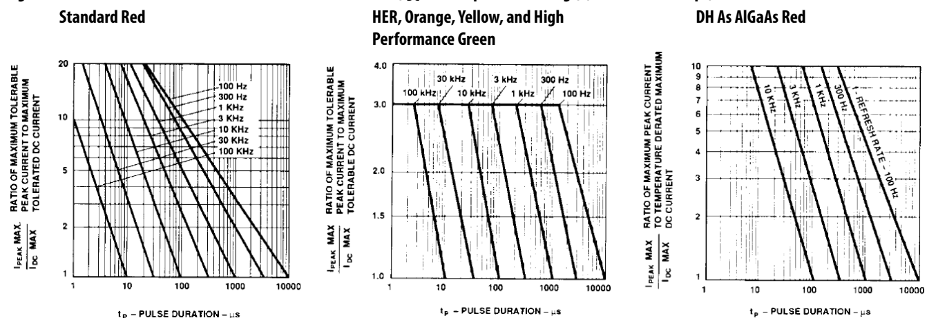
Figure 7: Maximum Tolerable Peak Current vs. Pulse Duration ( I_{DC} Max. as per Max. ratings) (non-resistor lamps)
