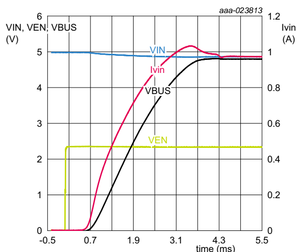
Fig 15. Typical 100 uF enable time versus inrush current
