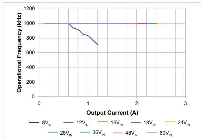
Figure 16 — Switching Frequency vs. Output Current @ 50V OUT
