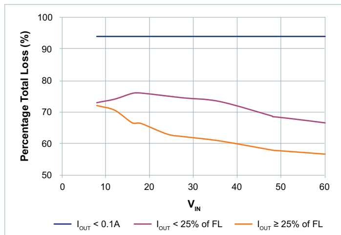
Figure 46 — V_{OUT} = 28V
