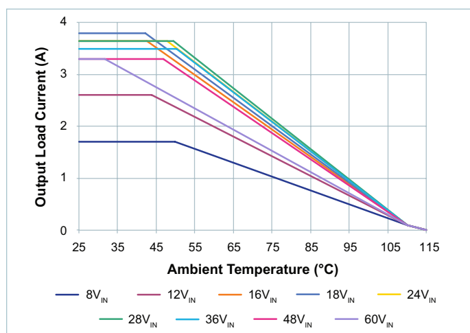
Figure 54 — Thermal de-rating for PI3740-00 evaluation board at V_{OUT} = 36V , 0LFM
