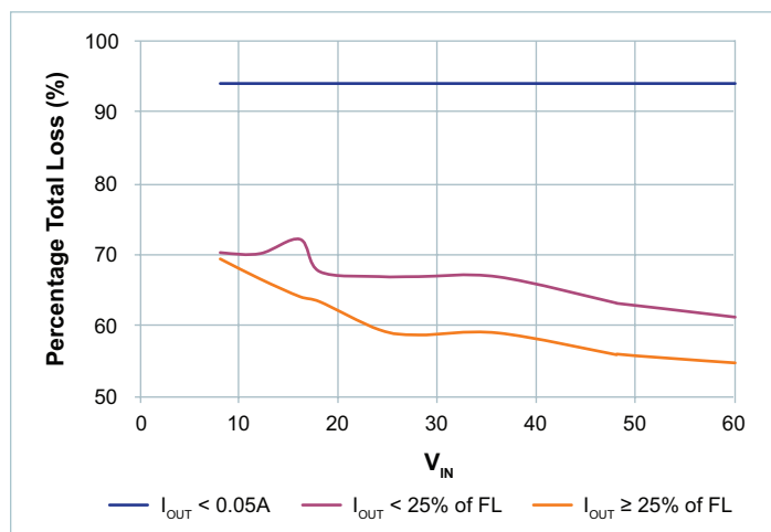
Figure 47 — V_{OUT} = 36V
