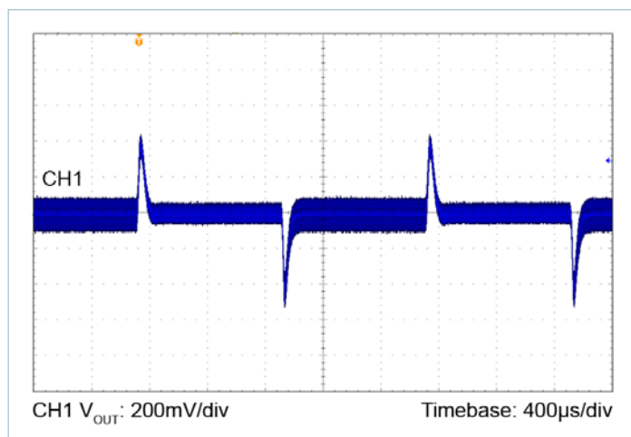
Figure 28 — 24V_{IN} to 36V_{OUT} , C_{OUT} = 8 \times 10\mu\text{F} Ceramic 1.5A to 3.0A Load Step, 0.1A/μs
