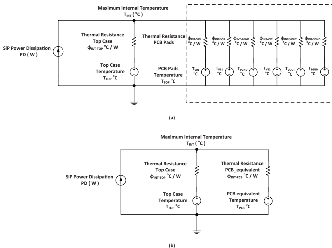
Figure 40 — PI3740-00 SiP Thermal Model (a) and its simplified version (b).
