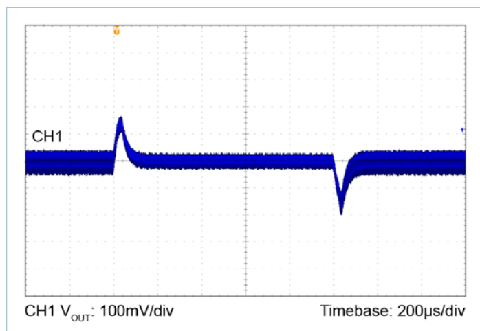
Figure 25 — 24V_{IN} to 12V_{OUT} , C_{OUT} = 8 \times 10\mu\text{F} Ceramic 3.38A to 6.75A Load Step, 0.1A/μs
