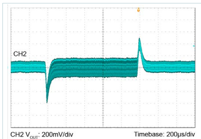
Figure 29 — 24V_{IN} to 50V_{OUT} , C_{OUT} = 8 \times 2.2\mu\text{F} Ceramic 2.5A to 1.25A Load Step, 0.1A/μs
