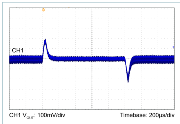
Figure 24 — 24V_{IN} to 10V_{OUT} , C_{OUT} = 8 \times 10\mu\text{F} Ceramic 3.5A to 7.0A Load Step, 0.1A/μs
