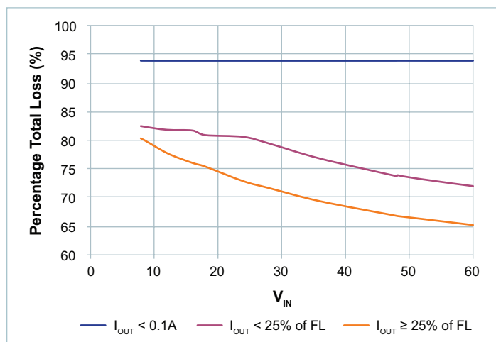
Figure 43 — V_{OUT} = 12V
