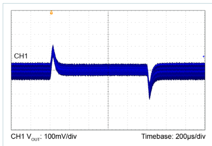
Figure 26 — 24V_{IN} to 24V_{OUT} , C_{OUT} = 8 \times 10\mu\text{F} Ceramic 2.5A to 5.0A Load Step, 0.1A/μs
