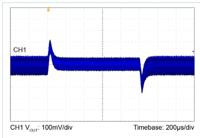
Figure 27 — 24V_{IN} to 28V_{OUT} , C_{OUT} = 8 \times 10\mu\text{F} Ceramic 2.25A to 4.5A Load Step, 0.1A/μs
