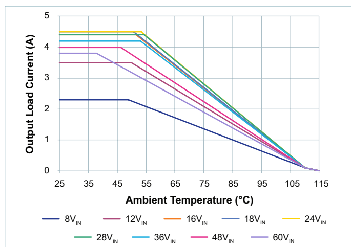
Figure 53 — Thermal de-rating PI3740-00 evaluation board at V_{OUT} = 28V , 0LFM
