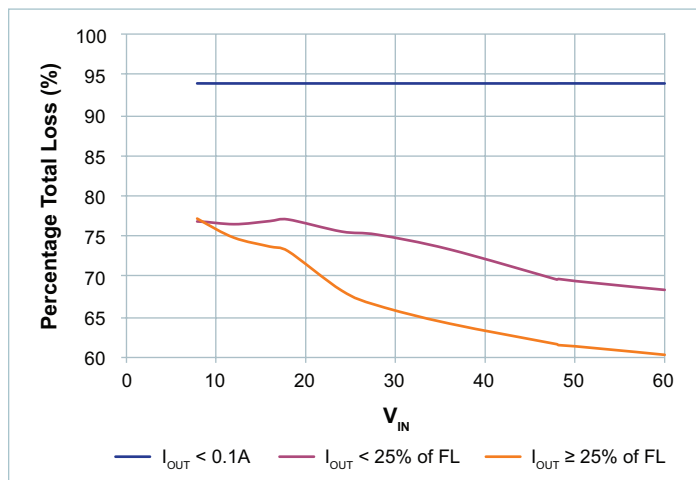
Figure 44 — V_{OUT} = 18V
