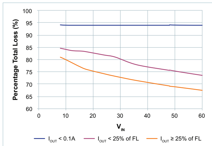
Figure 42 — V_{OUT} = 10V
