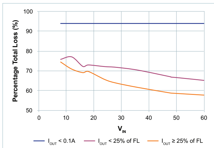
Figure 45 — V_{OUT} = 24V
