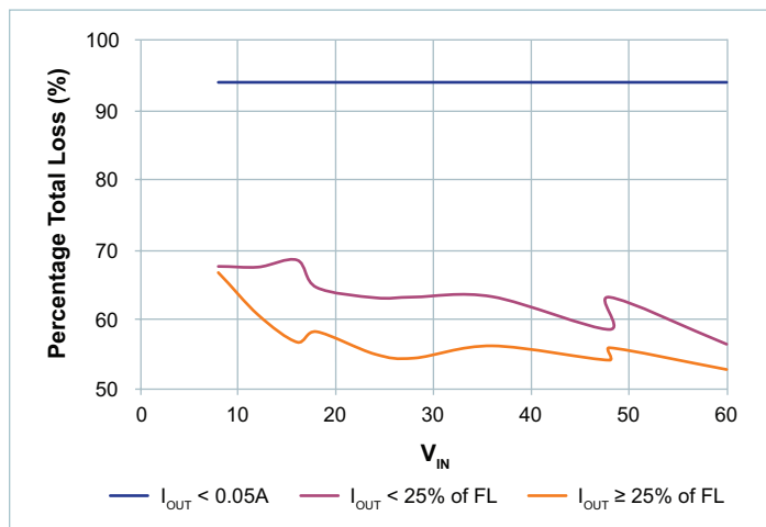
Figure 48 — V_{OUT} = 50V
