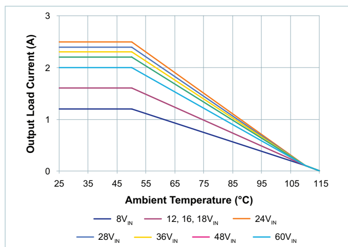
Figure 55 — Thermal de-rating for PI3740-00 evaluation board at V_{OUT} = 50V , 0LFM
