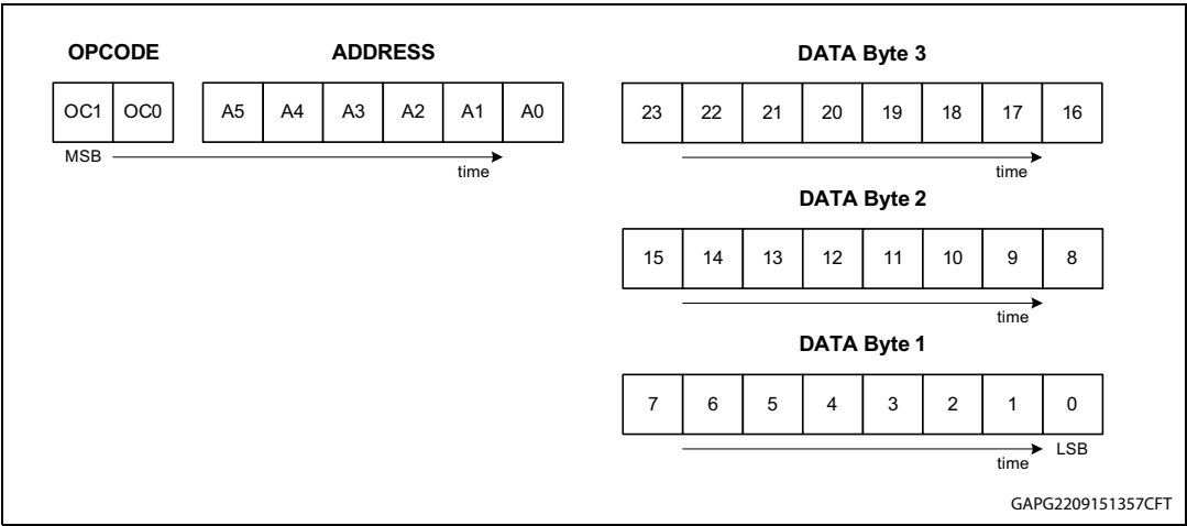
Figure 56. SDI Frame
