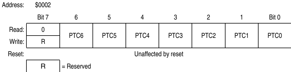
Figure 10-8. Port C Data Register (PTC)
