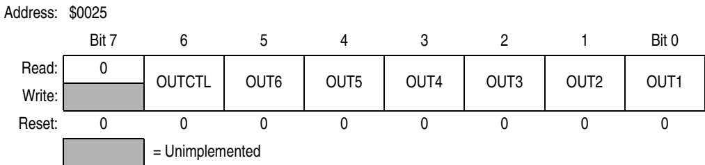
Figure 12-46. PWM Output Control Register (PWMOUT)
