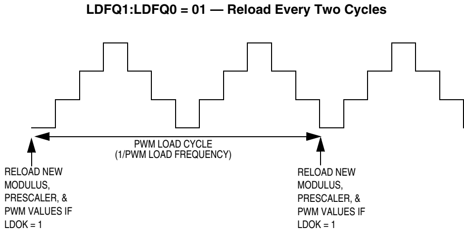
Figure 12-48. PWM Load Cycle/Frequency Definition
