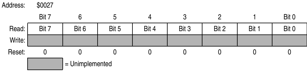
Figure 12-34. PWM Counter Register Low (PCNTL)
