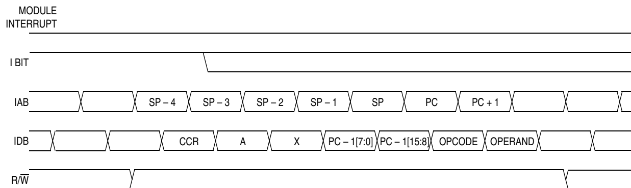
Figure 14-9. Interrupt Recovery
