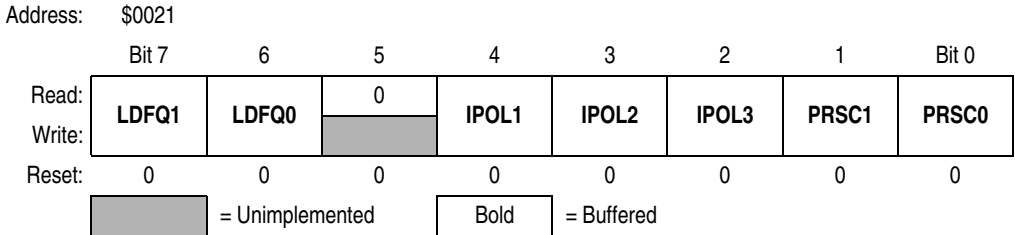
Figure 12-40. PWM Control Register 2 (PCTL2)
