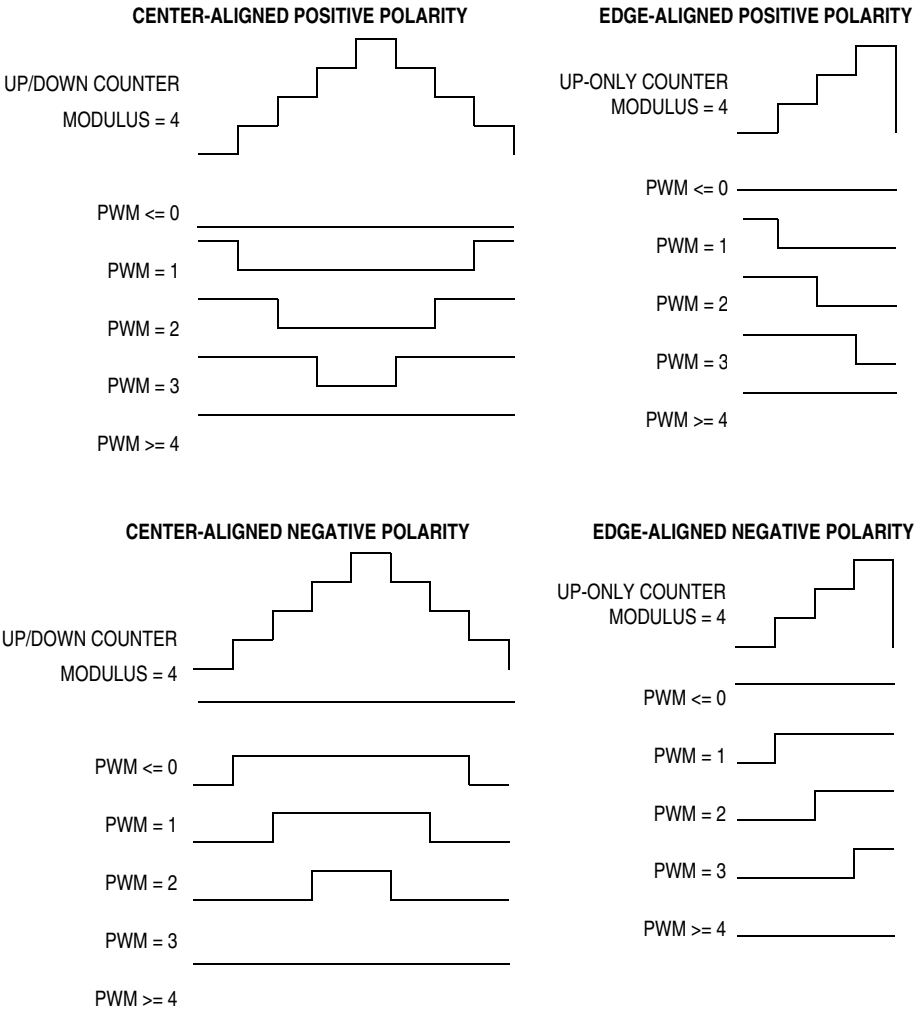
Figure 12-21. PWM Polarity
