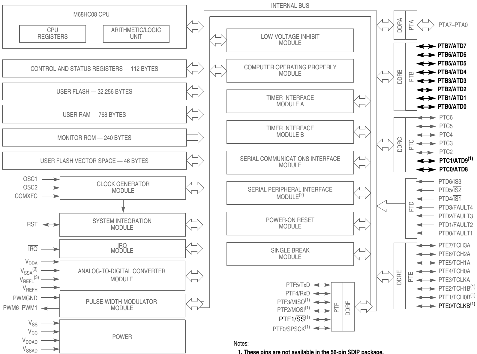
Figure 3-1. Block Diagram Highlighting ADC Block and Pins
