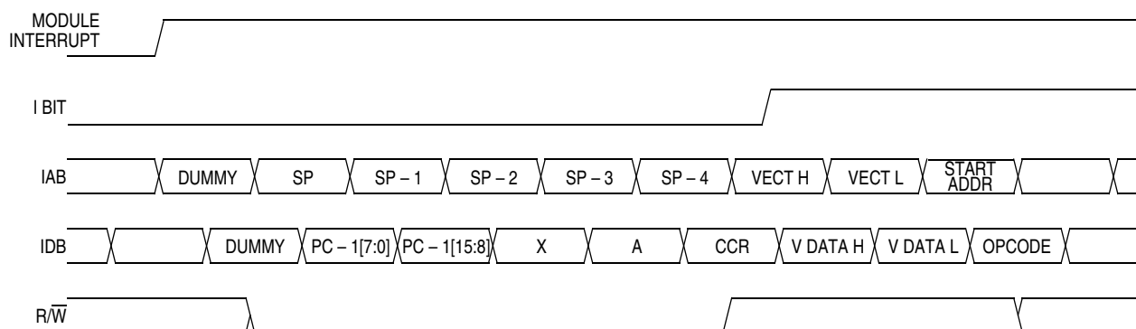
Figure 14-7. Interrupt Entry
