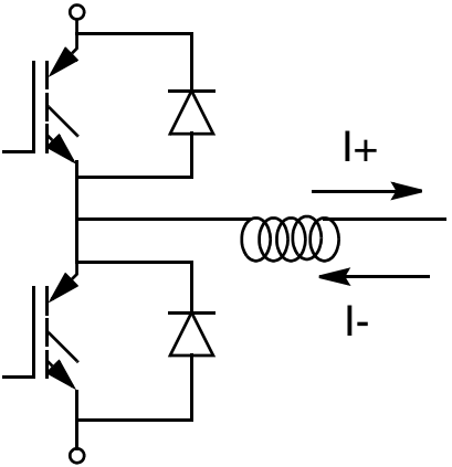
Figure 12-19. Current Convention
