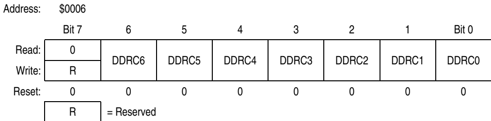
Figure 10-9. Data Direction Register C (DDRC)
