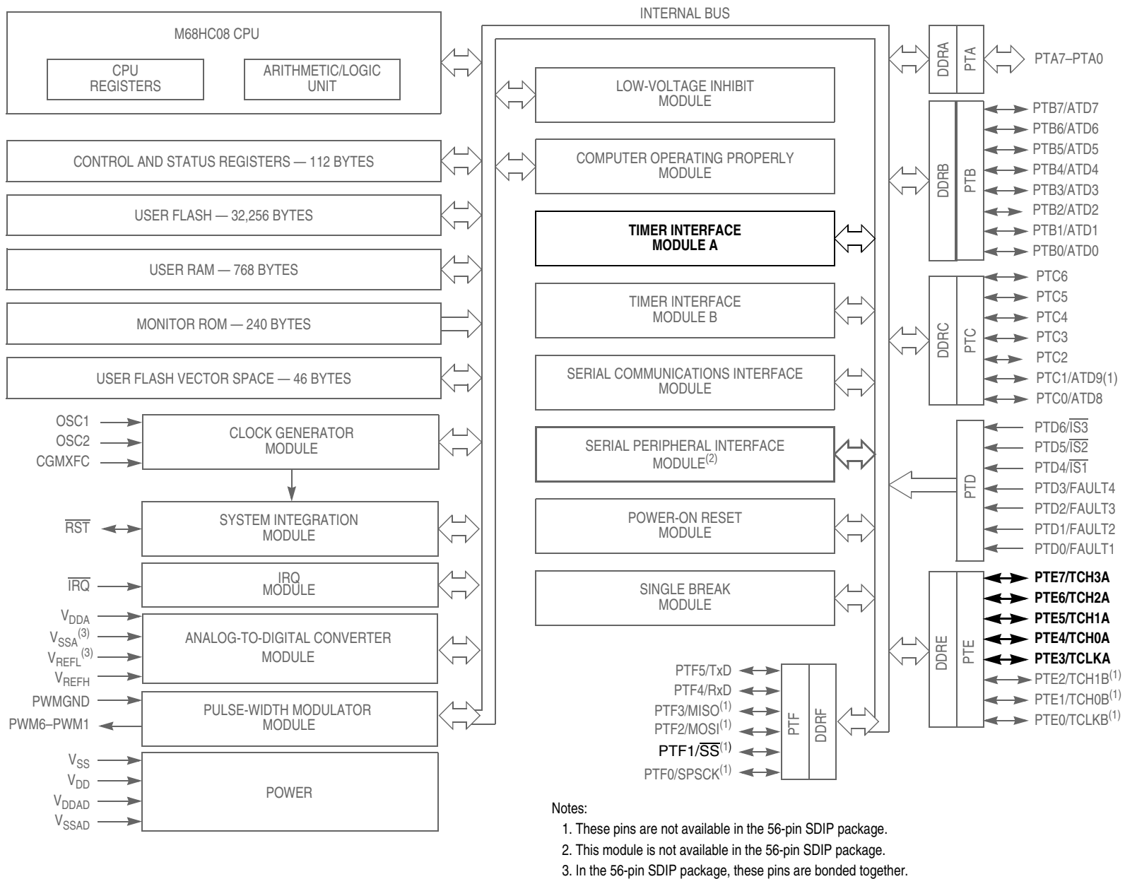
Figure 16-1. Block Diagram Highlighting TIMA Block and Pins
