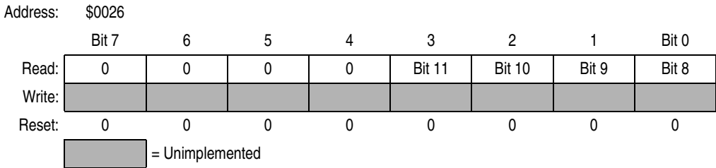
Figure 12-33. PWM Counter Register High (PCNTH)
