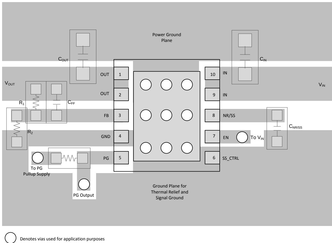
Figure 42. TPS7A91 Example Layout
