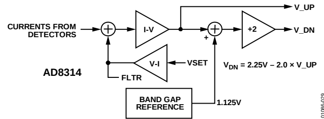
Figure 29. Output Interfaces
