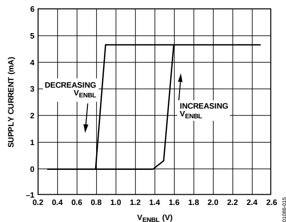
Figure 15. Supply Current vs. ENBL Voltage, V_S = 3V
