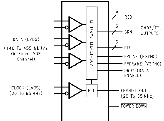
Figure 3. DS90CF364
