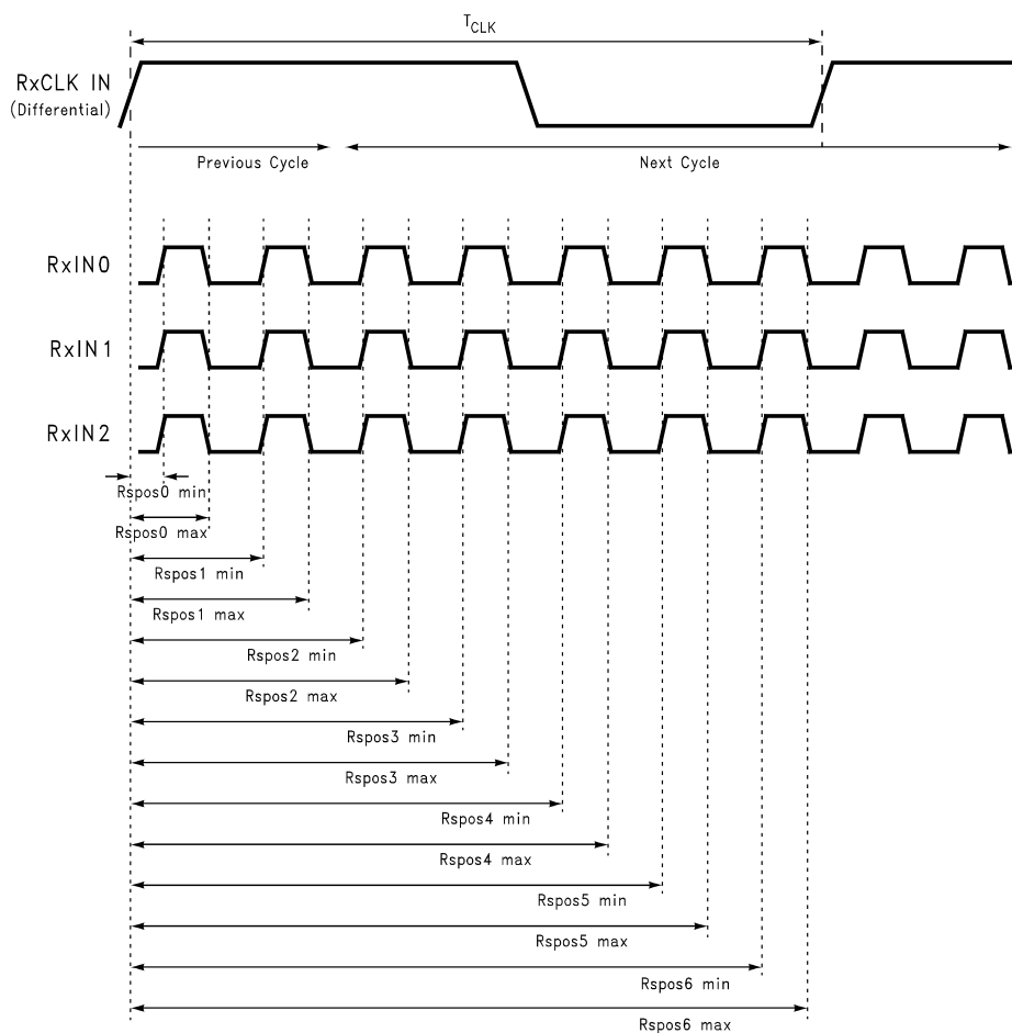
Figure 21. Receiver LVDS Input Strobe Position
