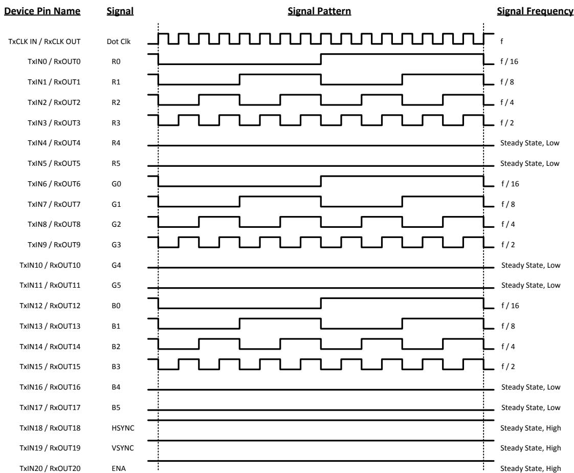
Figure 4. "Worst Case" Test Pattern
