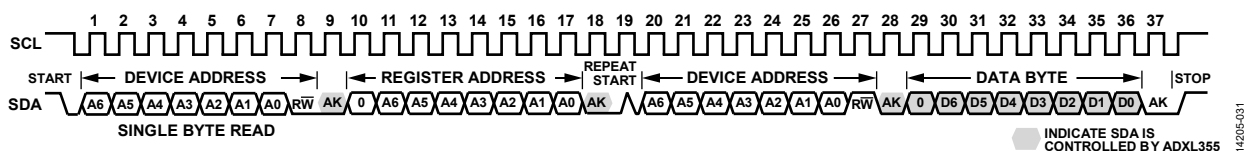
Figure 70. I 2 C Timing Diagram—Single-Byte Read
