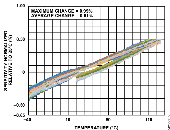
Figure 19. ADXL354 Sensitivity Normalized Relative to 25°C vs. Temperature Z-Axis
