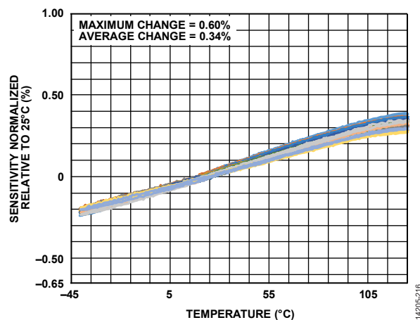
Figure 17. ADXL354 Sensitivity Normalized Relative to 25°C vs. Temperature X-Axis
