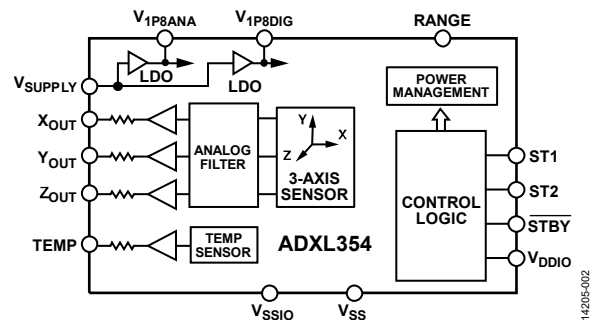
Figure 1. ADXL354
