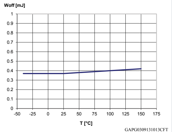
Figure 30. W_{off} vs. T_{case}
