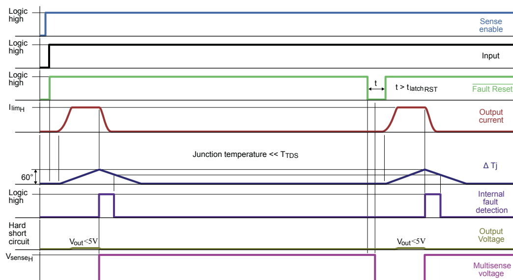
Figure 10. Latch functionality - behavior in hard short-circuit condition ( T_{AMB} \ll T_{TSD} )
