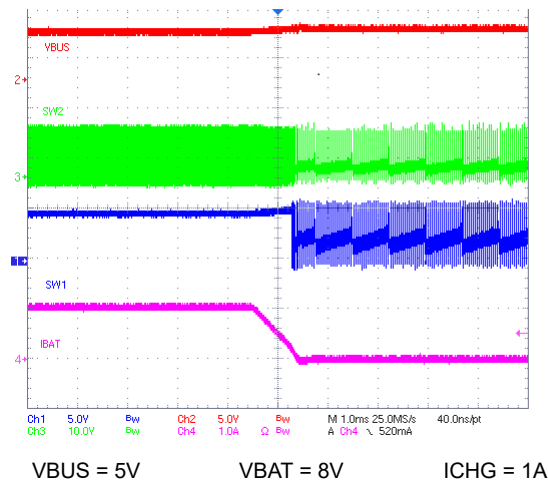
Figure 9-6. Charge Disable
