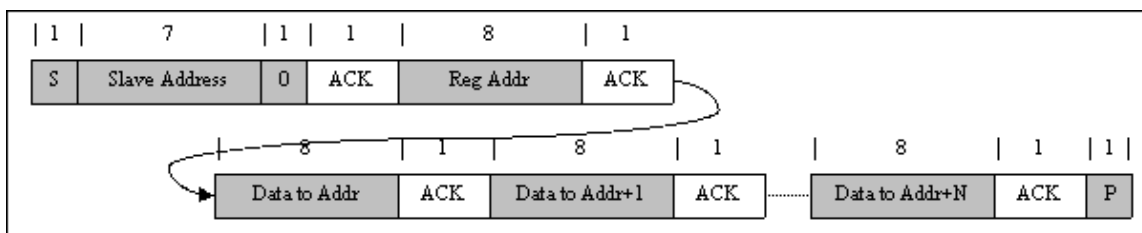
Figure 8-22. Multi-Write
