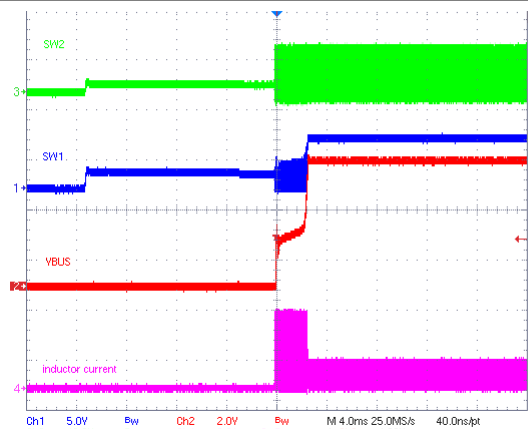
Figure 9-13. OTG Startup at 500-mA Load
