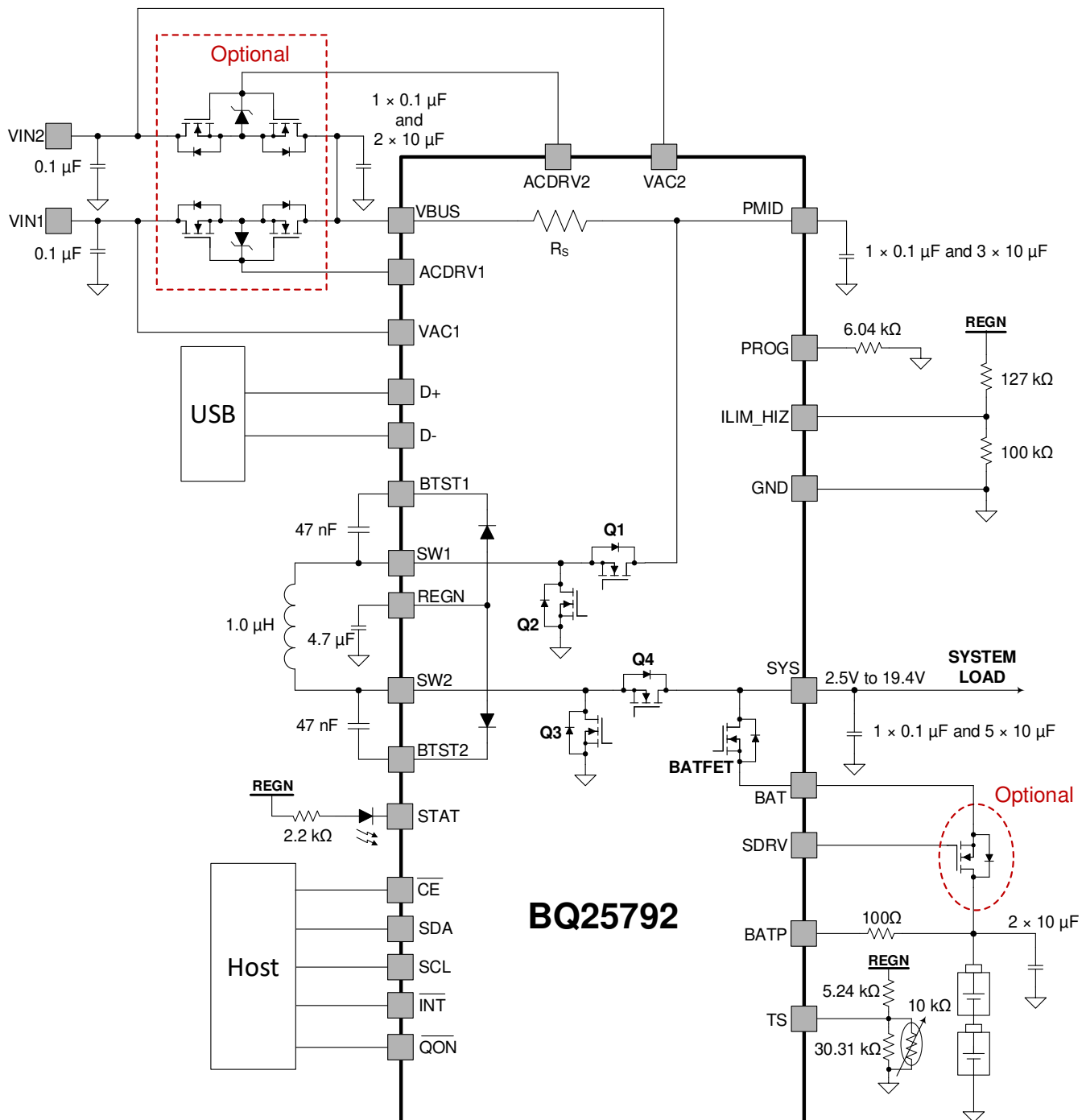
Figure 9-1. BQ25792 Application Diagram with Two Input Sources and Ship FET
