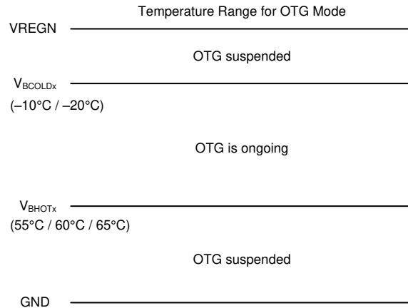
Figure 8-12. TS Pin Thermistor Sense Threshold in OTG Mode
