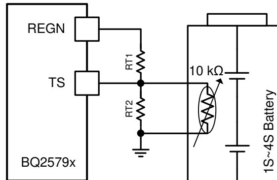
Figure 8-11. TS Resistor Network
