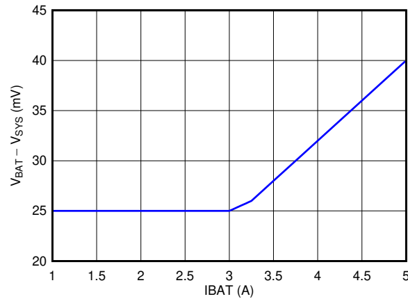
Figure 8-7. BATFET I-V Curve
