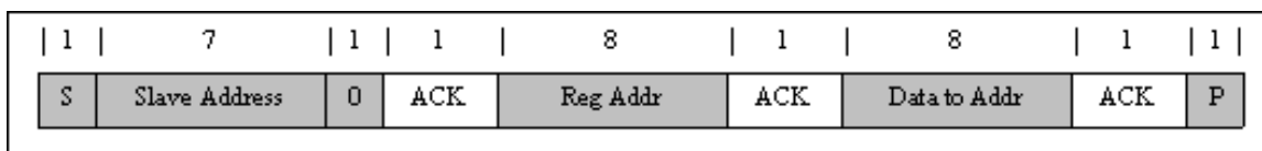
Figure 8-20. Single Write
