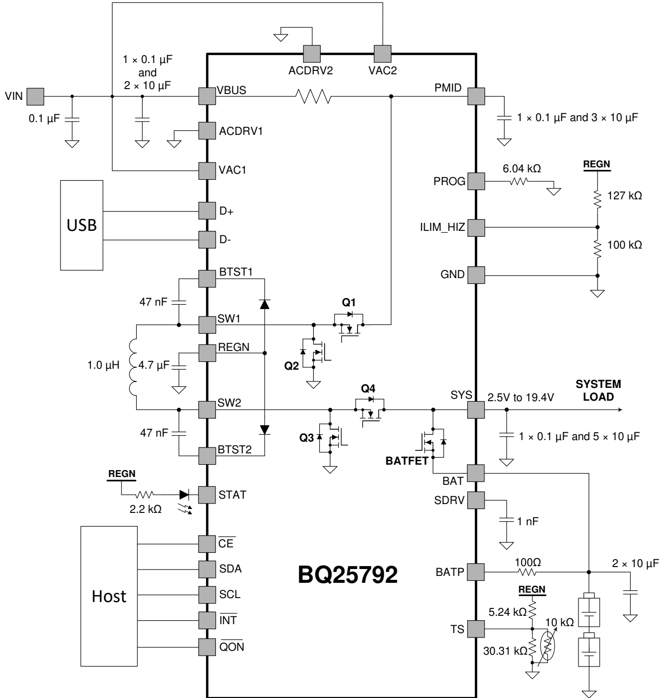
Figure 9-2. BQ25792 Application Diagram with Single Input Source and No Ship FET
