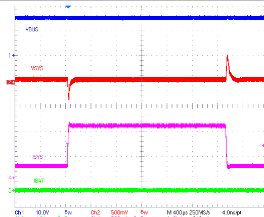
Figure 9-14. VSYS Load Transient Response
