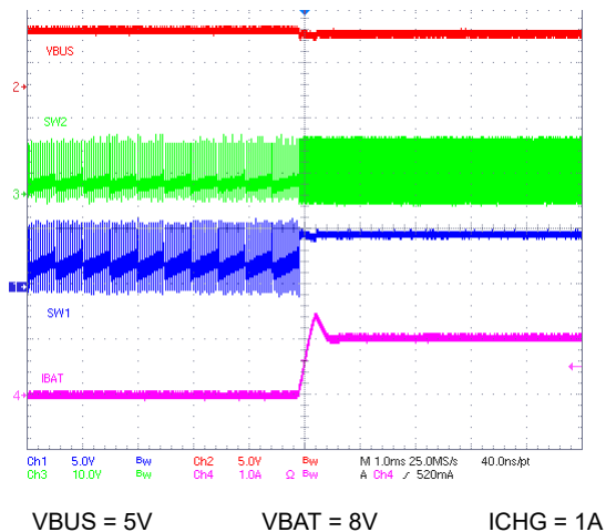
Figure 9-5. Charge Enable
