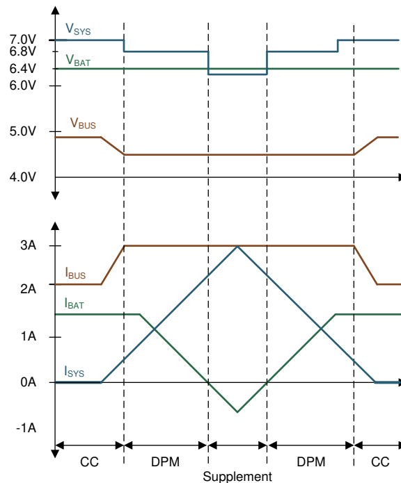
Figure 8-8. DPM Response
