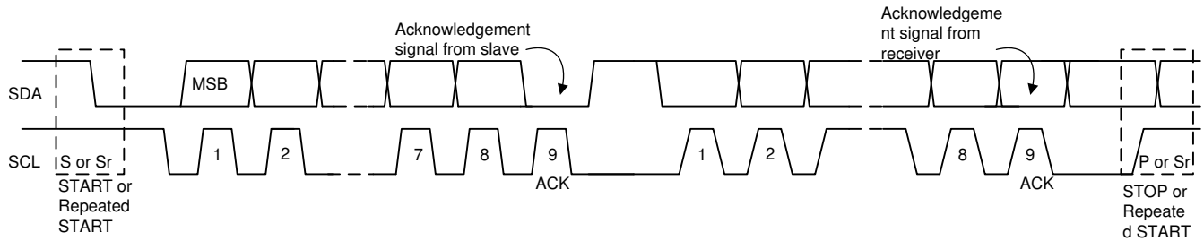
Figure 8-17. Data Transfer on the I²C Bus
