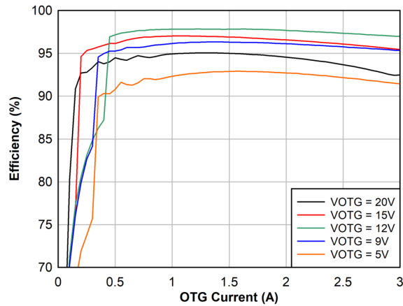
Figure 7-11. 2s Battery OTG Efficiency, 750 kHz
