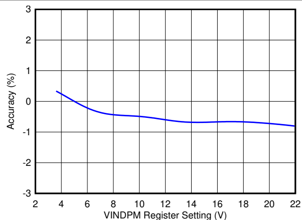
Figure 7-18. Input Voltage Regulation (VINDPM) Accuracy
