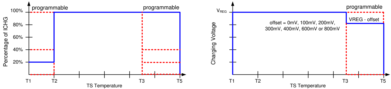
Figure 8-10. TS Charging Values
