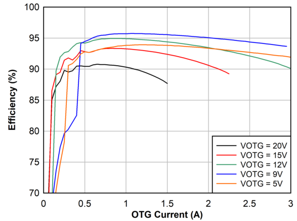
Figure 7-12. 2s Battery OTG Efficiency, 1.5 MHz
