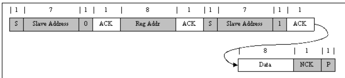
Figure 8-21. Single Read
