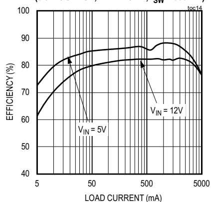
EFFICIENCY vs. LOAD CURRENT (1.8V OUTPUT, PFM MODE, f_{SW} = 400kHz )
