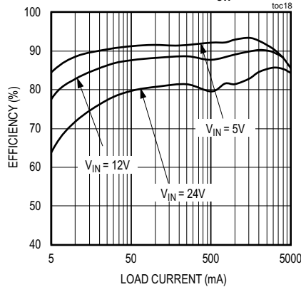
EFFICIENCY vs. LOAD CURRENT (2.5V OUTPUT, PFM MODE, f_{SW} = 400kHz )
