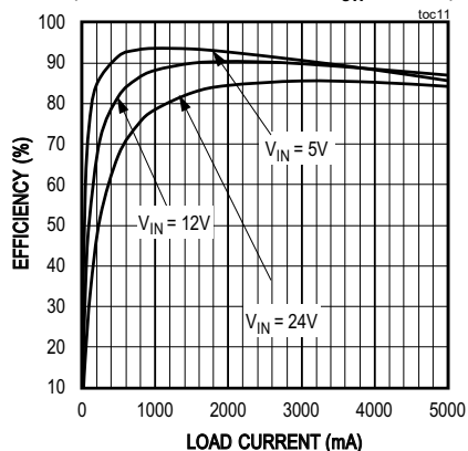
EFFICIENCY vs. LOAD CURRENT (0.9V OUTPUT, PFM MODE, f_{SW} = 300kHz )
