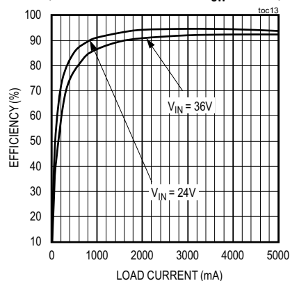
EFFICIENCY vs. LOAD CURRENT (1.5V OUTPUT, PFM MODE, f_{SW} = 400kHz )
