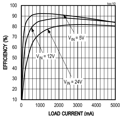
EFFICIENCY vs. LOAD CURRENT (12V OUTPUT, PWM MODE, f_{SW} = 900kHz )
