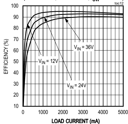
EFFICIENCY vs. LOAD CURRENT (1.2V OUTPUT, PFM MODE, f_{SW} = 400kHz )
