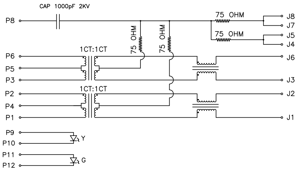
SCHEMATIC
