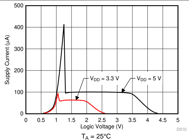
Figure 10. Supply Current vs Logic Voltage
