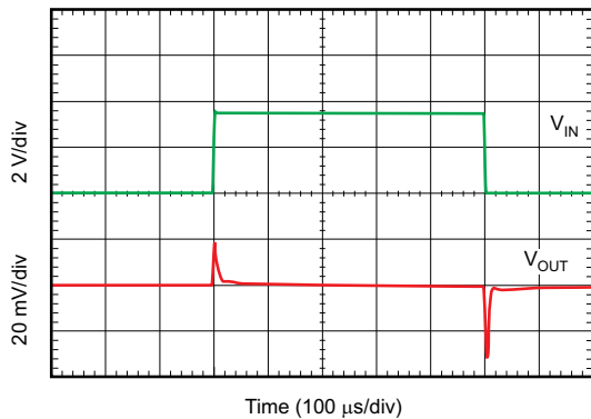
Figure 66. Line Transient Response
