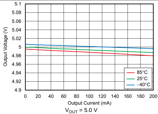
Figure 3. Load Regulation
