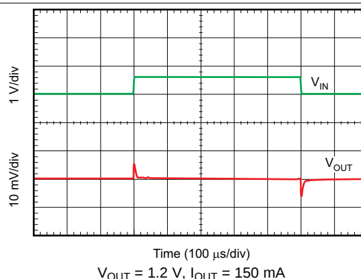
Figure 46. Line Transient Response
