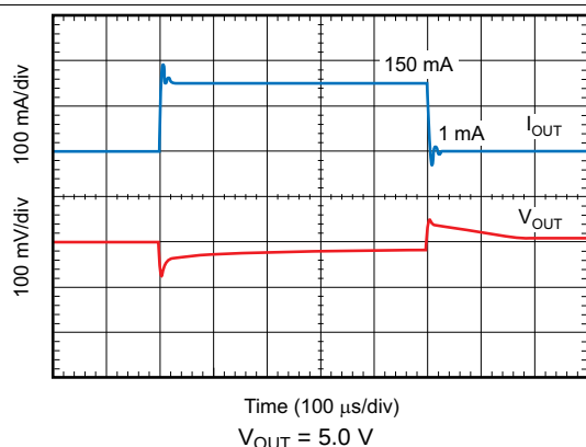
Figure 45. Load Transient Response
