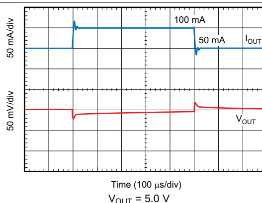
Figure 44. Load Transient Response
