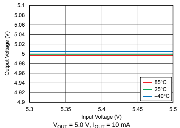
Figure 6. Line Regulation
