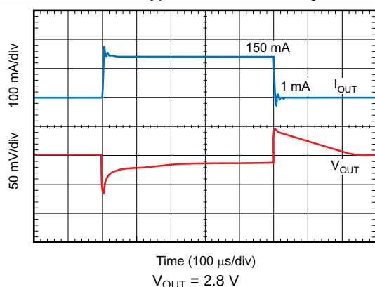
Figure 43. Load Transient Response
