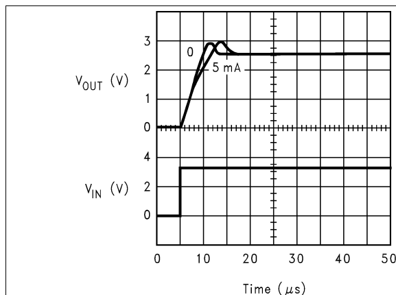
Figure 30. Start-Up Response
