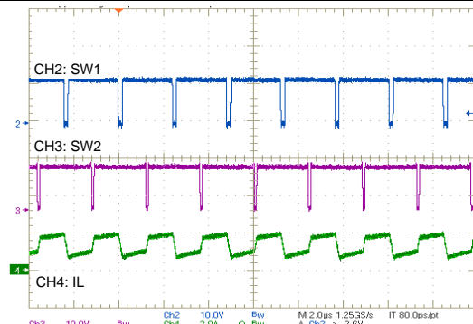
Figure 49. Switching During Buck Boost Mode
