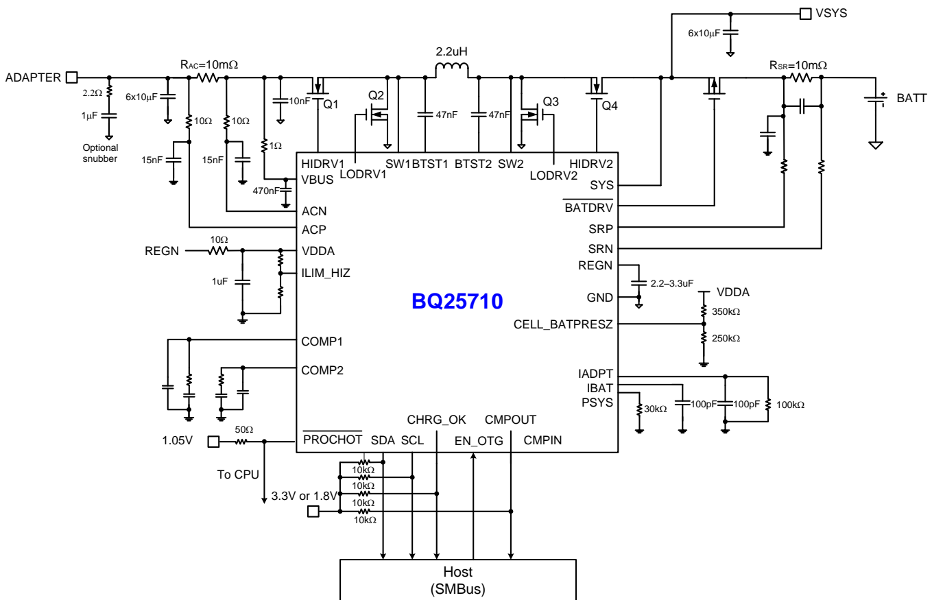
Figure 40. Application Diagram
