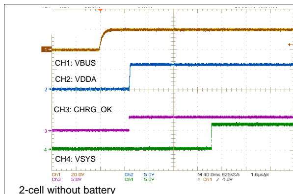
Figure 42. Power Up from 20 V
