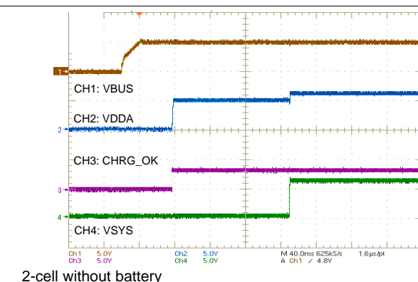
Figure 43. Power Up from 5 V
