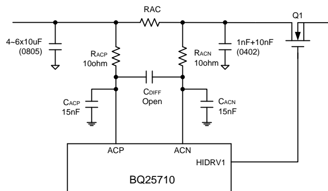
Figure 41. ACN-ACP Input Filter
