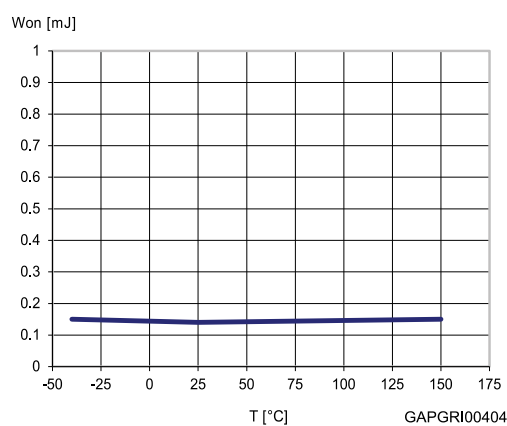
Figure 29: W_{on} vs. T_{case}
