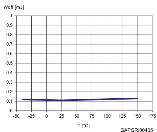
Figure 30: W_{off} vs. T_{case}
