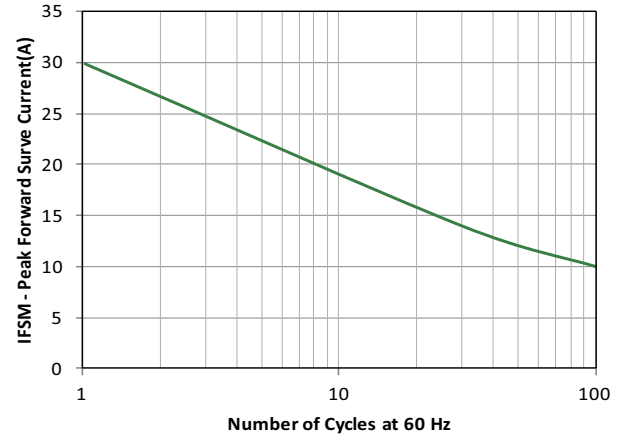
Figure 8 - Maximum Non-Repetitive Forward Surge Current Uni-Directional Only
