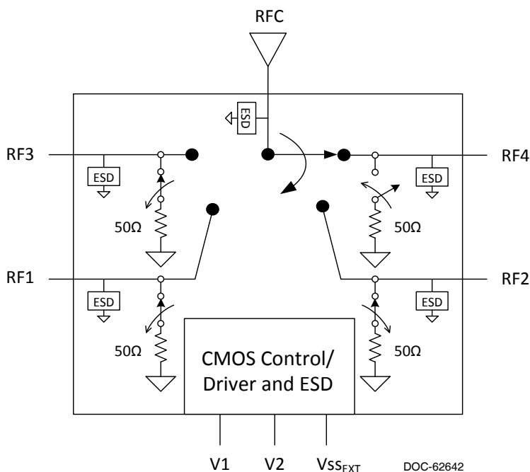
Figure 1. Functional Diagram
