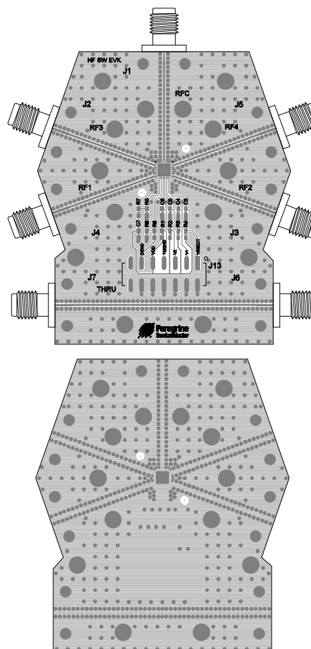
Figure 20. Evaluation Board Layout
