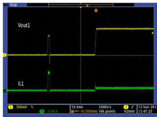
Figure 28. Hiccup Recover, Buck 1
