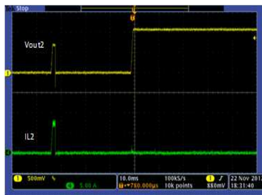
Figure 30. Hiccup Recover, Buck 2
