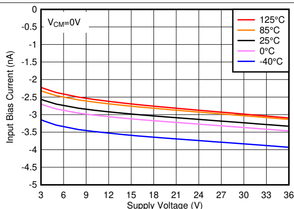
Figure 20. Input Bias Current vs. Supply Voltage
