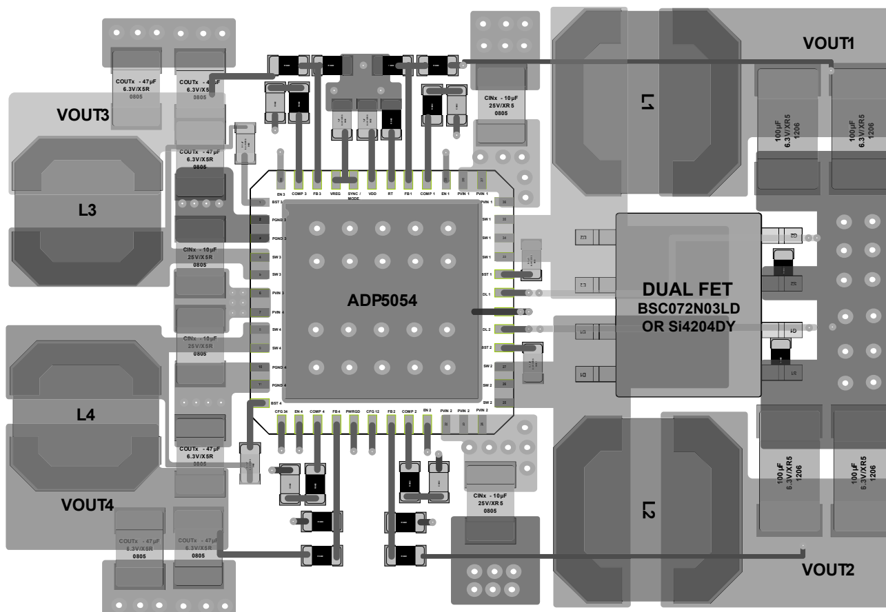
Figure 43. Typical PCB Layout for the ADP5054
