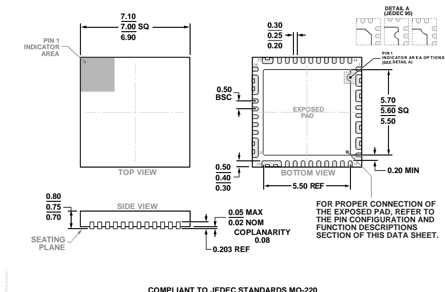
COMPLIANT TO JEDEC STANDARDS MO-220 Figure 45. 48-Lead Lead Frame Chip Scale Package [LFCSP] 7 mm × 7 mm Body and 0.75 mm Package Height with Fused Leads (CP-48-16) Dimensions shown in millimeters
