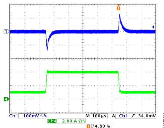
Figure 21. Channel 1/Channel 2 Load Transient, 1A to 4A, V_{IN} = 12V , V_{OUT} = 3.3V , f_{SW} = 600kHz , L = 2.2\mu H , C_{OUT} = 47\mu F \times 2 , Channel 1 = V_{OUTx} , Channel 4 = I_{OUTx}
