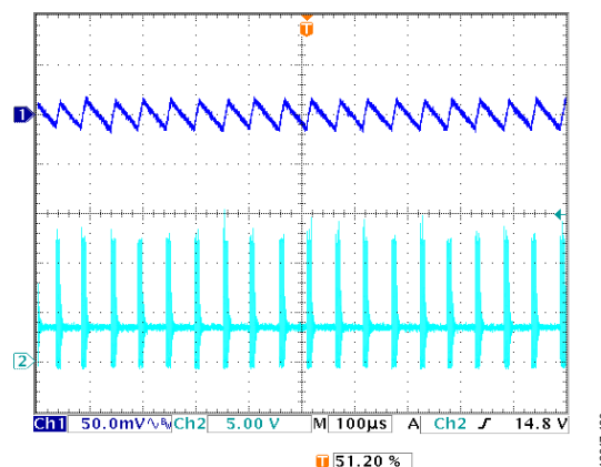
Figure 20. Steady State Waveform at Light Load, V_{IN} = 12V , V_{OUT} = 3.3V , I_{OUT} = 30mA , f_{SW} = 600kHz , L = 4.7\mu H , C_{OUT} = 47\mu F \times 2 , Automatic PWM/PSM Mode, Channel 1 = V_{OUTx} , Channel 2 = SWx
