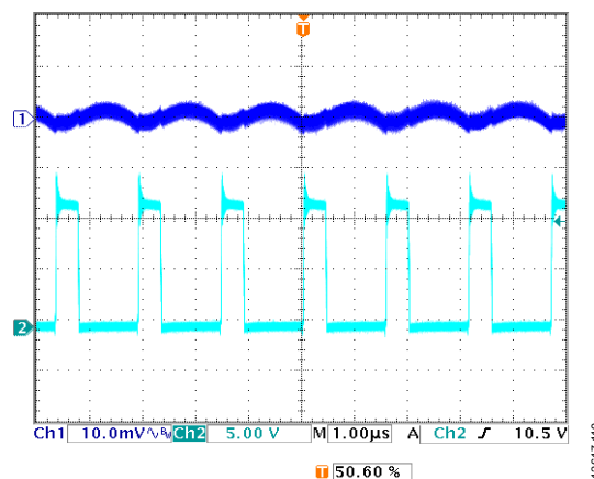
Figure 19. Steady State Waveform at Heavy Load, V_{IN} = 12V , V_{OUT} = 3.3V , Output Load Current ( I_{OUT} ) = 3A, f_{SW} = 600kHz , L = 4.7\mu H , C_{OUT} = 47\mu F \times 2 , FPWM Mode, Channel 1 = V_{OUTx} , Channel 2 = SWx
