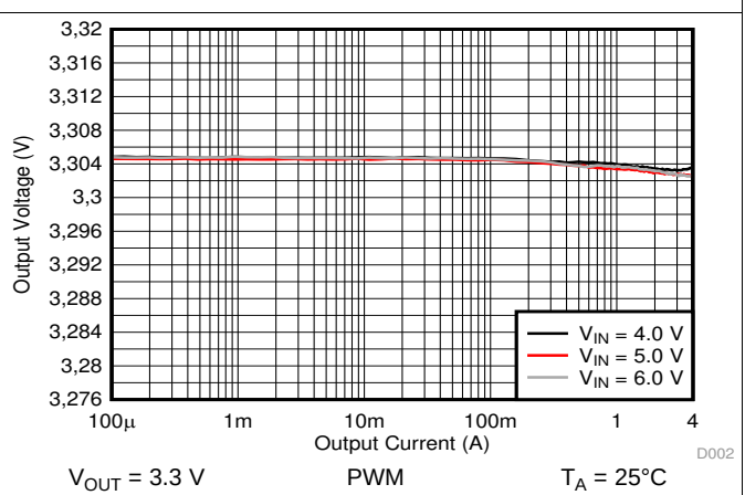
Figure 17. Output Voltage versus Output Current
