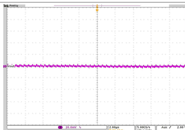
Figure 51. Output Voltage Ripple
