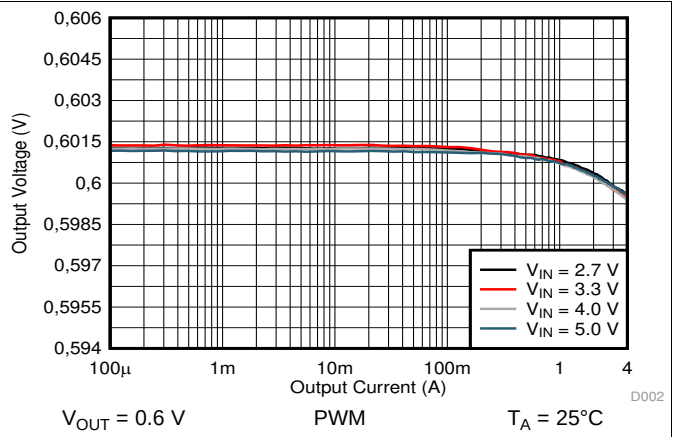
Figure 25. Output Voltage versus Output Current
