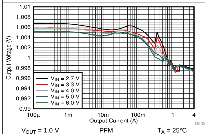
Figure 22. Output Voltage versus Output Current
