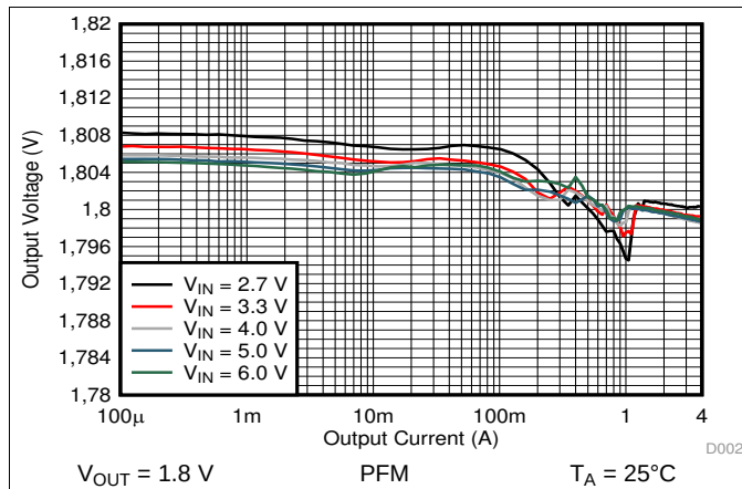
Figure 18. Output Voltage versus Output Current
