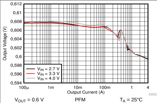
Figure 24. Output Voltage versus Output Current
