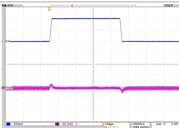
Figure 38. Line Transient Response
