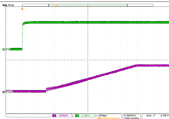
Figure 56. Start-Up Timing
