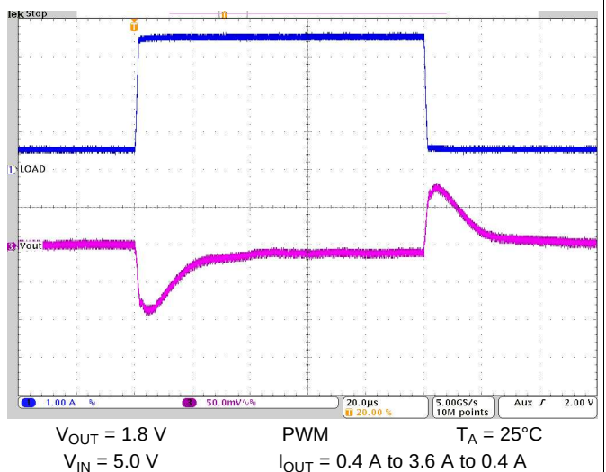
Figure 29. Load Transient Response
