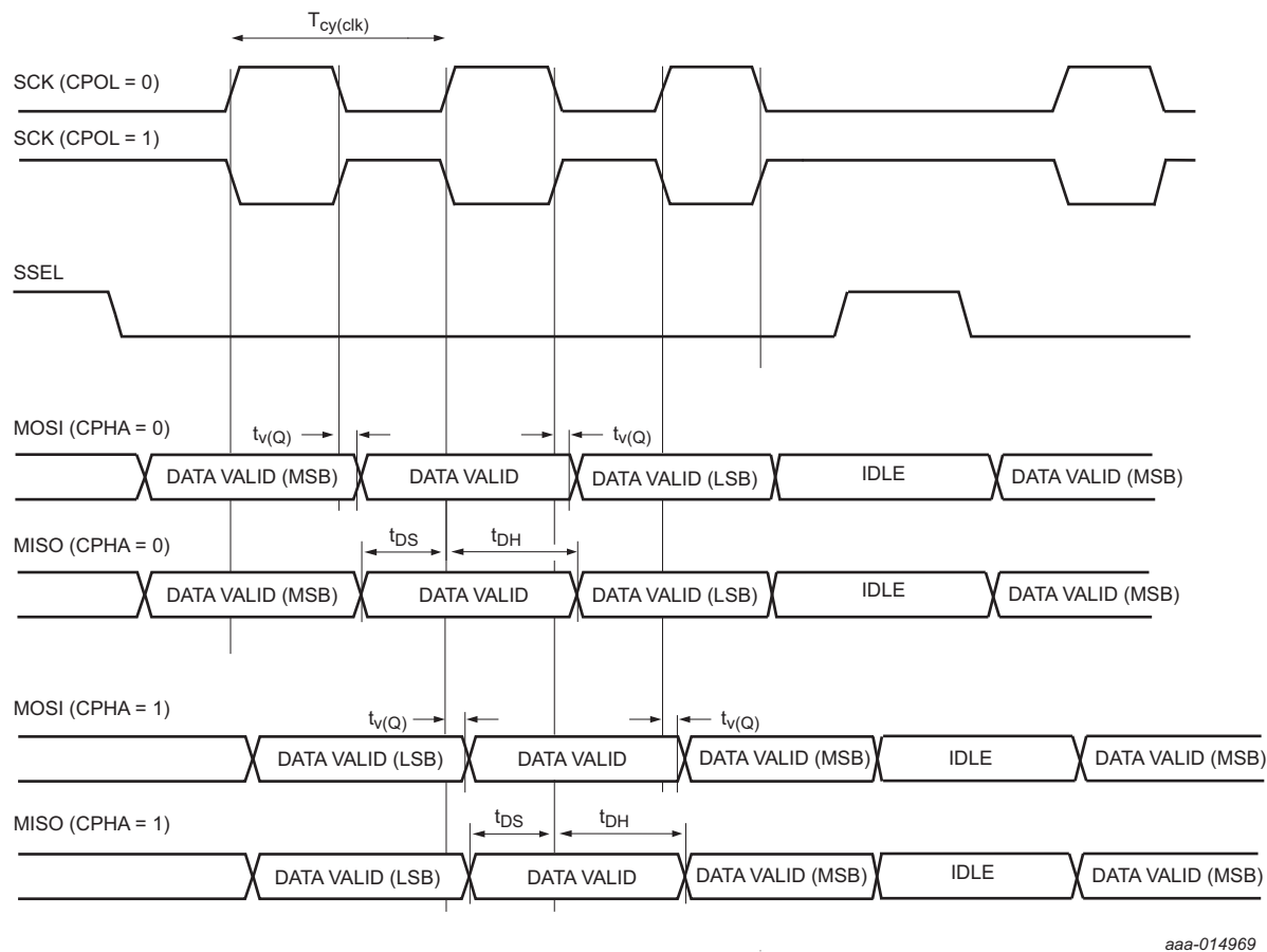
Fig 31. SPI master timing
