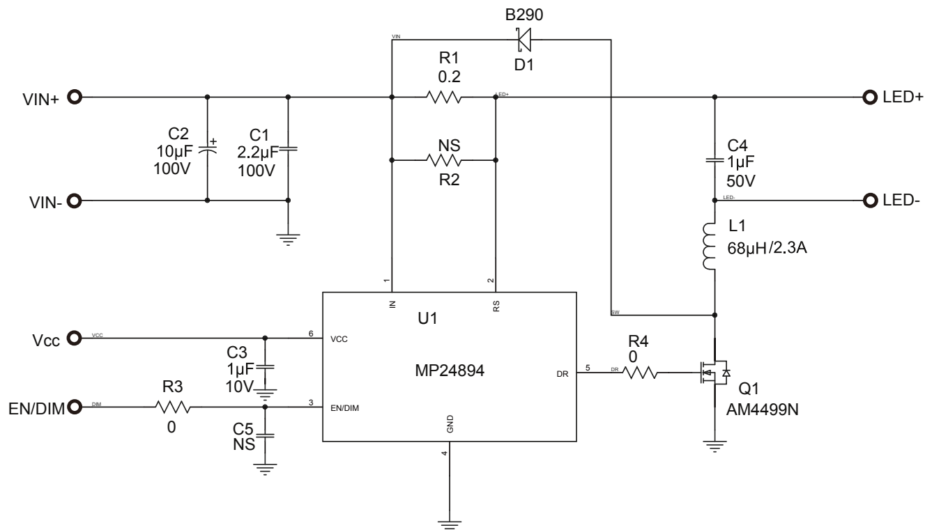
Figure 2: Application Circuit
