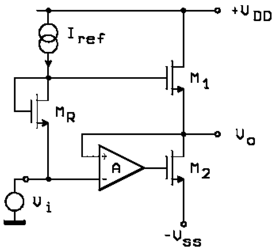
Figure 16. Principle schematic of a DMOS unity-gain buffer
