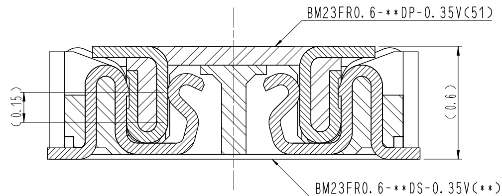
ENGAGEMENT FIGURE (50:1)
