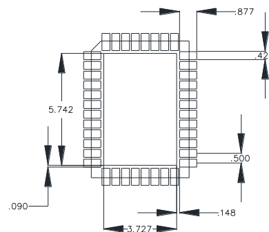
SOLDER MASK
