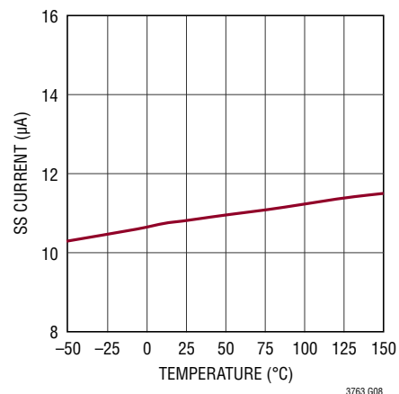
SS Current
