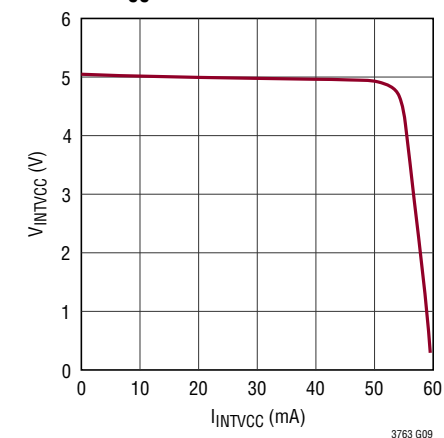
INTVCC Current Limit
