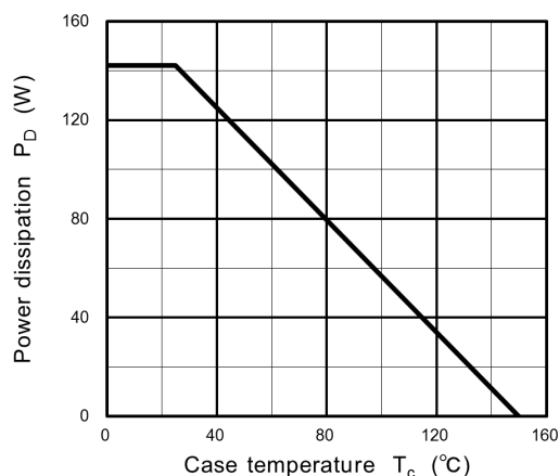
Fig. 8.14 P_D - T_c (Guaranteed Maximum)
