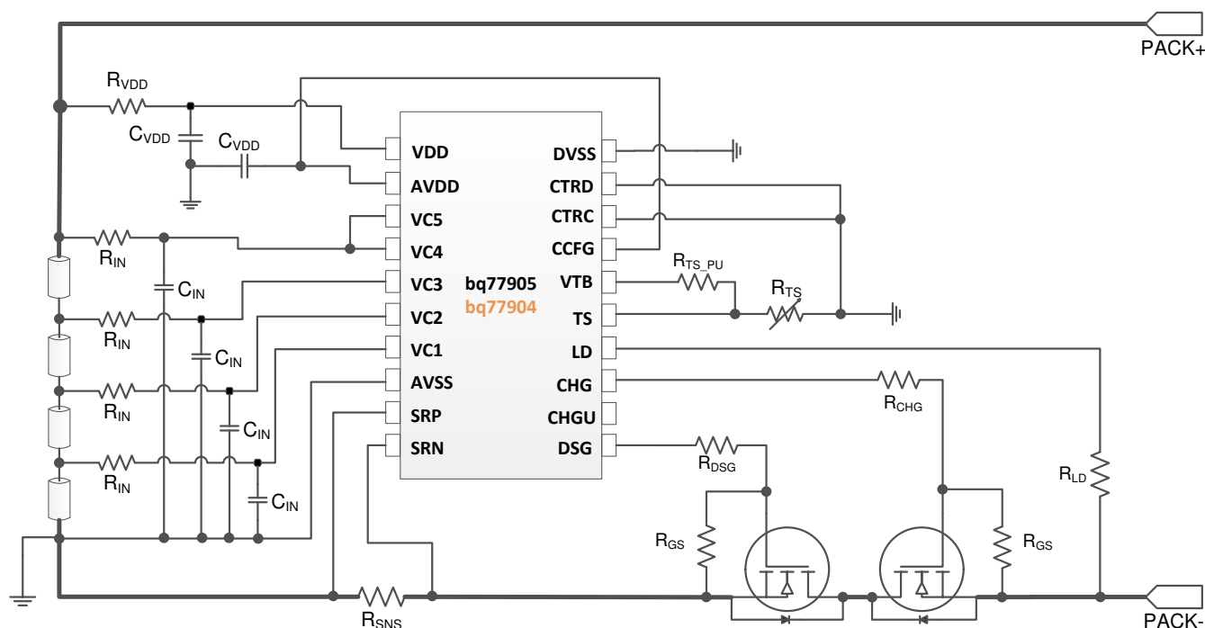
Figure 9-9. BQ77904 and BQ77905 with Four Cells
