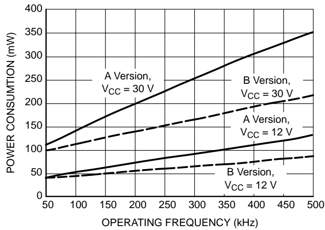
Figure 69. IC Power Consumption as a Function of Frequency for C DRV = 1 nF, R MIN_TON = R MIN_TOFF = 5 kΩ
