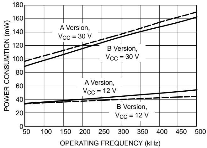
Figure 68. IC Power Consumption as a Function of Frequency for C DRV = 0 nF, R MIN_TON = R MIN_TOFF = 5 kΩ
