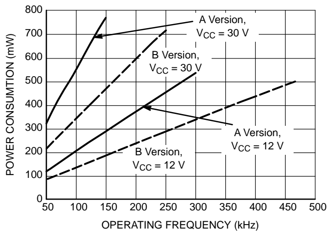
Figure 70. IC Power Consumption as a Function of Frequency for C DRV = 10 nF, R MIN_TON = R MIN_TOFF = 5 kΩ
