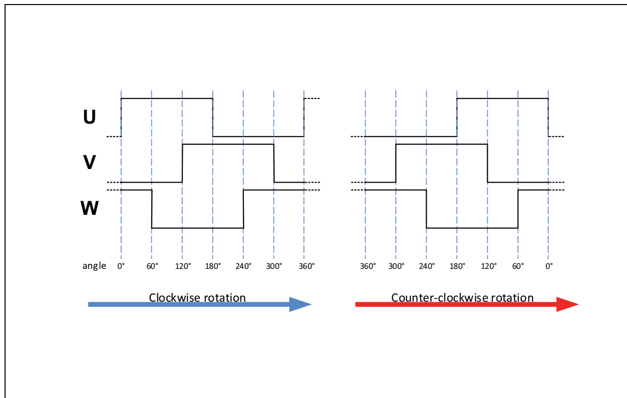
Figure 33: UVW Signals
