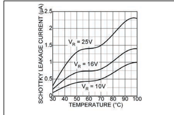
FIGURE 2-10: Schottky Reverse Leakage Current.
