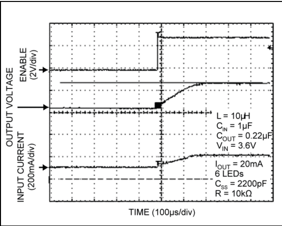
FIGURE 2-15: 6-Series LED Circuit with External Soft-Start.
