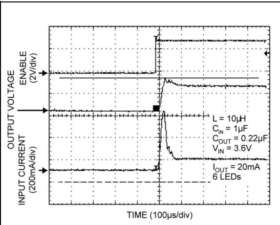
FIGURE 2-16: 6-Series LED Circuit without External Soft-Start.
